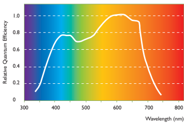
Light sensitivity curve of plants
